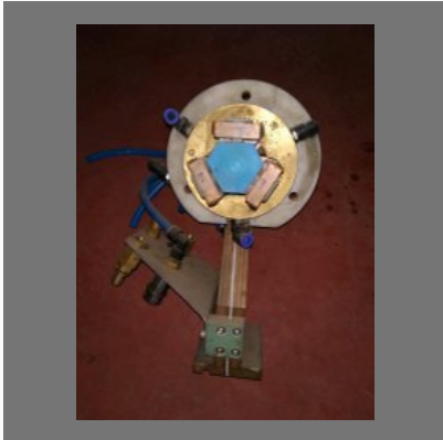
Induction Hardening Coil For Drive Shaft
