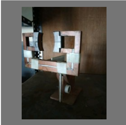
ferrotron Induction Hardening Coil
