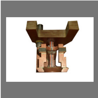
Single shot Induction hardening Coil
