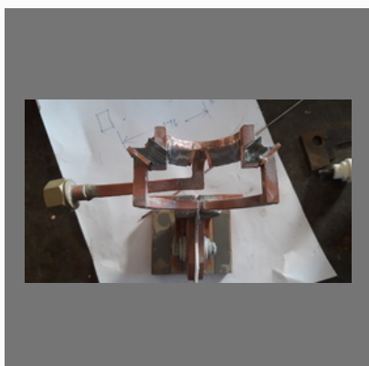
Induction brazing coil
