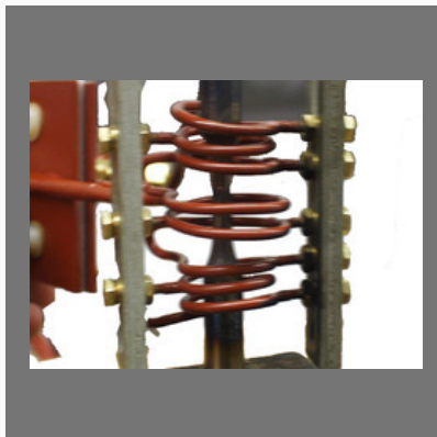
Copper Induction Coil for strength testing
